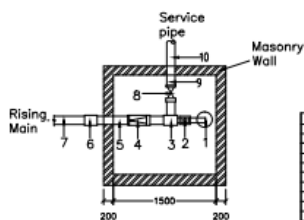
BOREHOLE CHAMBER PLAN
